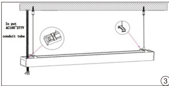
3. Connecting the AC cable with the electrical terminal of the lamp Inside.
