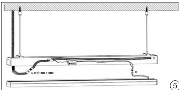
5. Connect the lamp with AC100-347V input.
