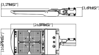
150W-200W
