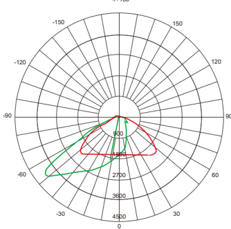
AST-S-G20-100WXYDA1
