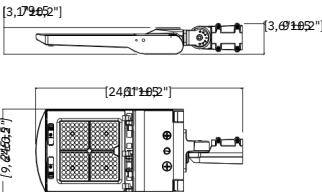
80W-100W
