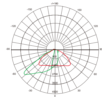
AST-S-G20-80WXYDA1
