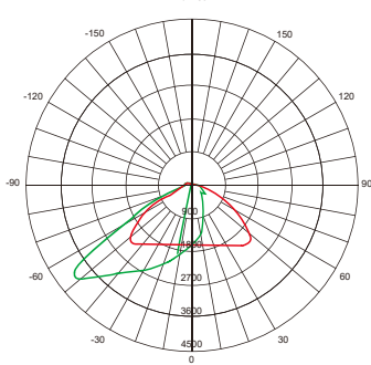
AST-S-G20-300WXYDA1
